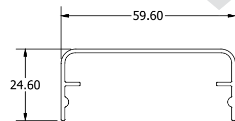
400K | 4.13 Kg/m Καπάκι κουπαστής Handrail Cover
