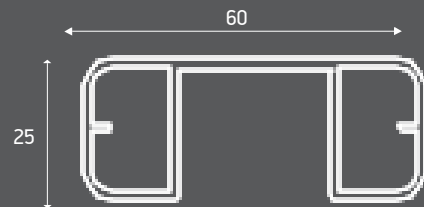
SD-6300N | 4,70kg ΚΟΥΠΑΣΤΗ 60x25mm Handrail 60x25mm
