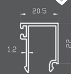
SD-6751 | 1,65kg ΚΑΠΑΚΙ ΓΙΑ 6750 32x25mm Cover for 6750 32x25mm
